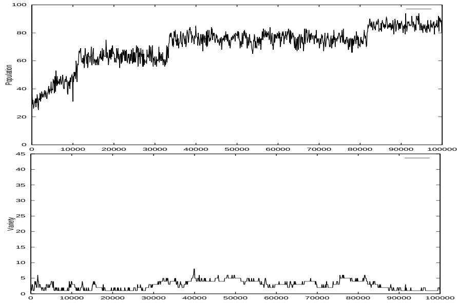
Figure 2: Population (total number of agents) and variety (number of distinct genomes) plots for run with probability of mutation equal to 0.001
