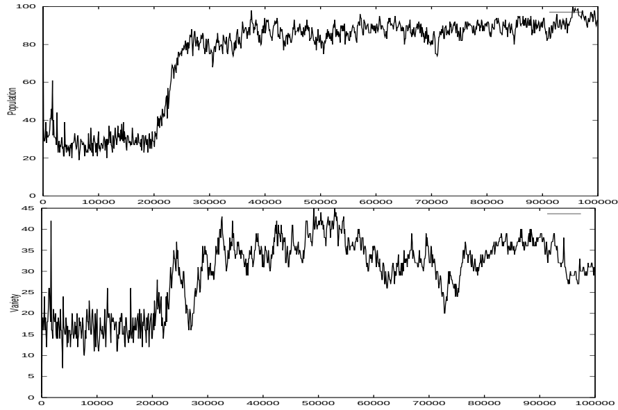
Figure 5: Population (total number of agents) and variety (number of distinct genomes) plots for run with probability of mutation equal to 0.05
