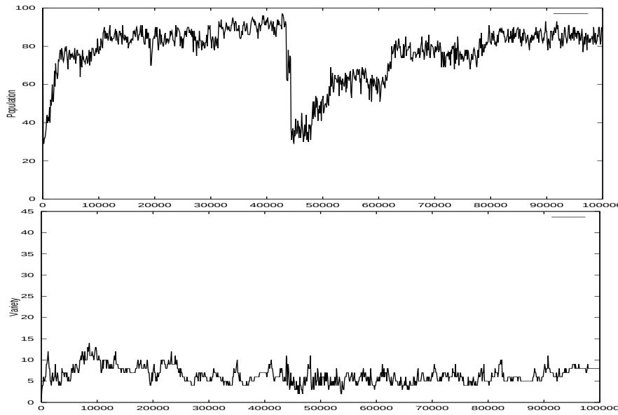
Figure 3: Population (total number of agents) and variety (number of distinct genomes) plots for run with probability of mutation equal to 0.005
