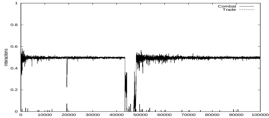
Figure 6: Relative frequencies of combat and trading interactions in the world reported on in Sections 4.3 and 5.2. Interactions are difficult to distinguish in the figure because of the density of the trading frequency time series. Trading is the interaction at the 0.5 level, except for the period from roughly 45000 to 50000, a period of combat.
