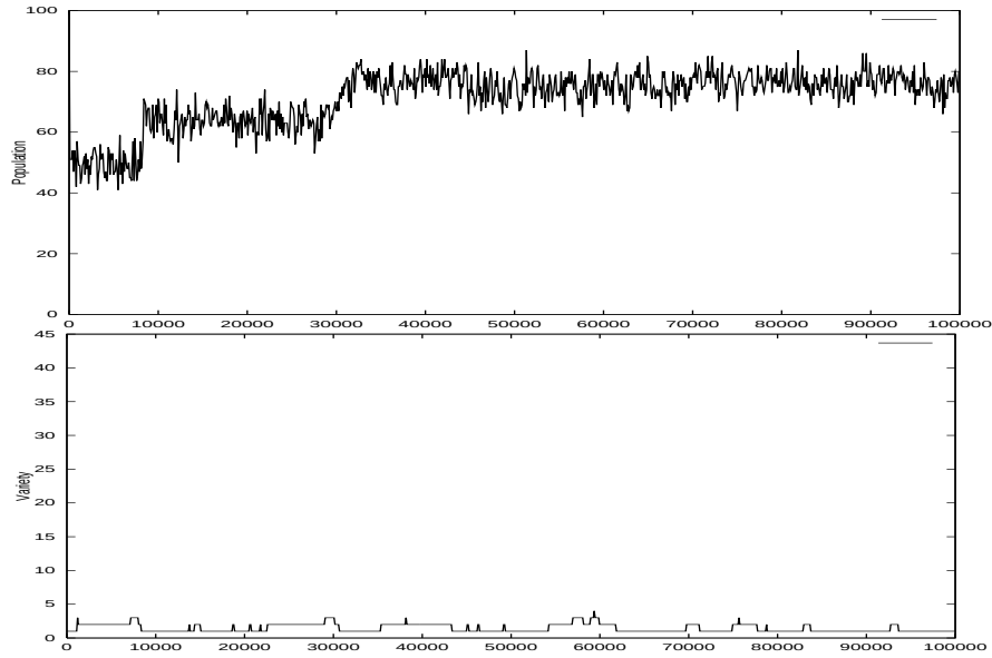
Figure 1: Population (total number of agents) and variety (number of distinct genomes) plots for run with probability of mutation equal to 0.0001
