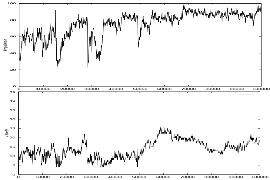
Figure 4: Population (total number of agents) and variety (number of distinct genomes) plots for run with probability of mutation equal to 0.01
